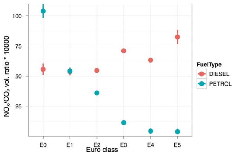
Fig. 7.5 Volume ratio of estimated NO x /CO 2 for petrol and diesel cars by Euro classification. The error bars show the 95 % confidence intervals in the mean (Source: Carslaw et al. 2011; https://uk-air.defra.gov.uk/assets/documents/reports/cat05/1108251149_110718_AQ0724_Final_report.pdf )
