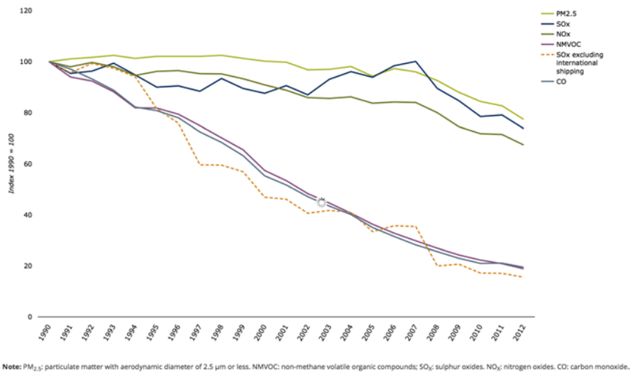
Fig. 7.3 Trends in emissions of air pollutants ( Source: European Environmental Agency 2015 )
