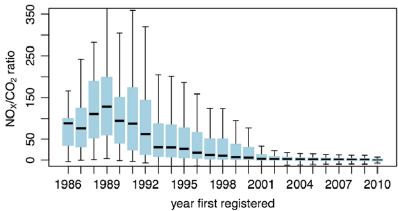
Fig. 7.4 Box plot of the volume ratio of NO x /CO 2 for petrol cars ( Source: Carslaw et al. 2011; https://uk-air.defra.gov.uk/assets/documents/reports/cat05/1108251149_110718_AQ0724_Final_report.pdf )
